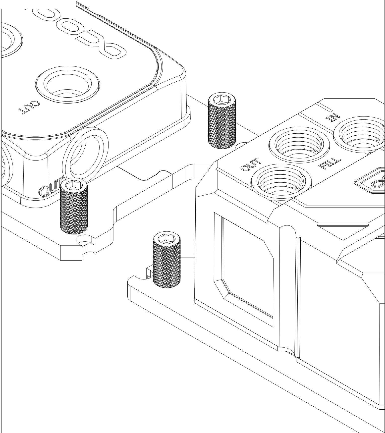
Alphacool XPX Pro/Eisbaer Pro LGA 4677 Mounting Bracket
